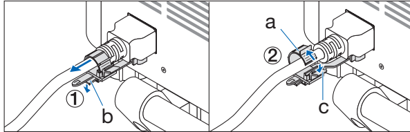
a: Clamber / b: Knob (power cord stopper) / c: Knob (clamber)
