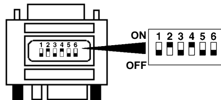
Figure 3-6. MAC Adaptor Switches
