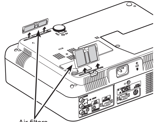
Air filters Pull up and remove.
