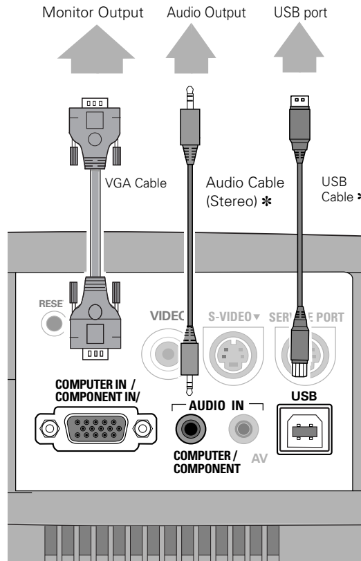
Terminals of the Projector
