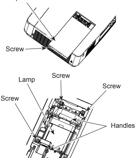
Lamp Cover
