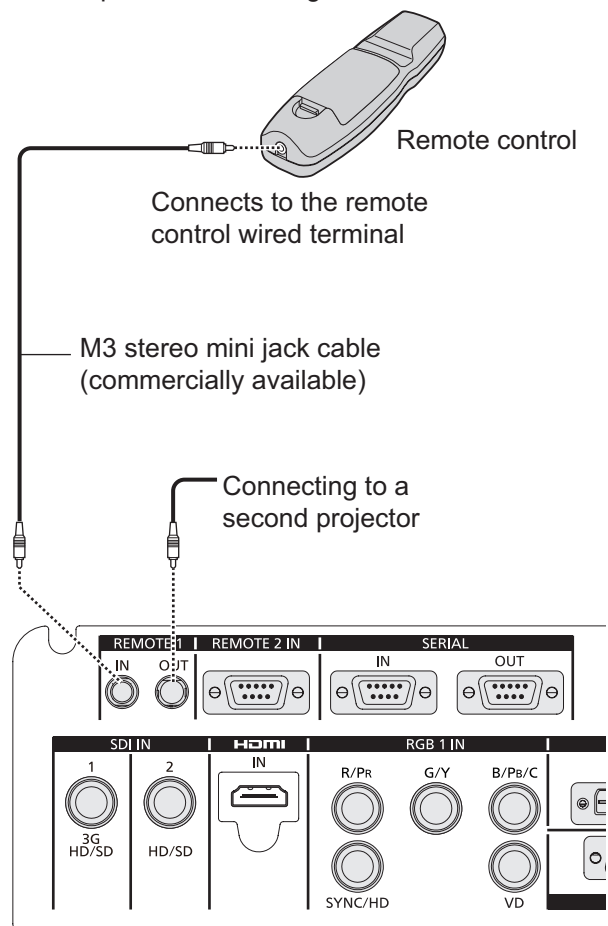
Connecting terminals
