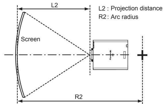
Horizontal arc correction (viewed from above)
