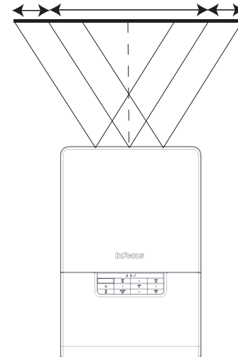
Horizontal Image Offset +/-15%
