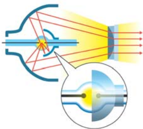
E-TORL: Epson-Twin Optimize Reflection Lamp
