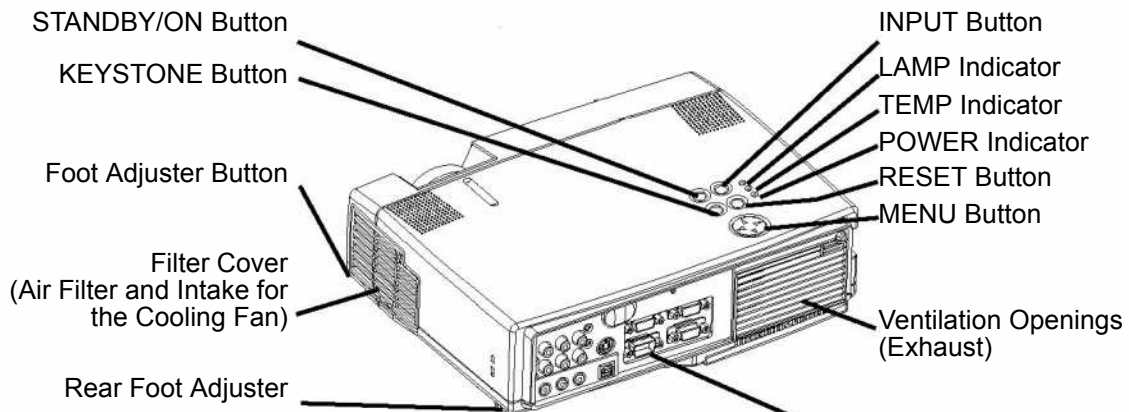
REAR/RIGHT VIEW OF THE PROJECTOR
