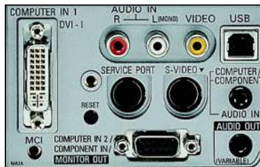
PLC-XU58 Terminal Input Panel
