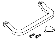
Carrying handle (24F39671) Screw (M4×2: 24N07501) Flathead screwdriver (24H51611)
