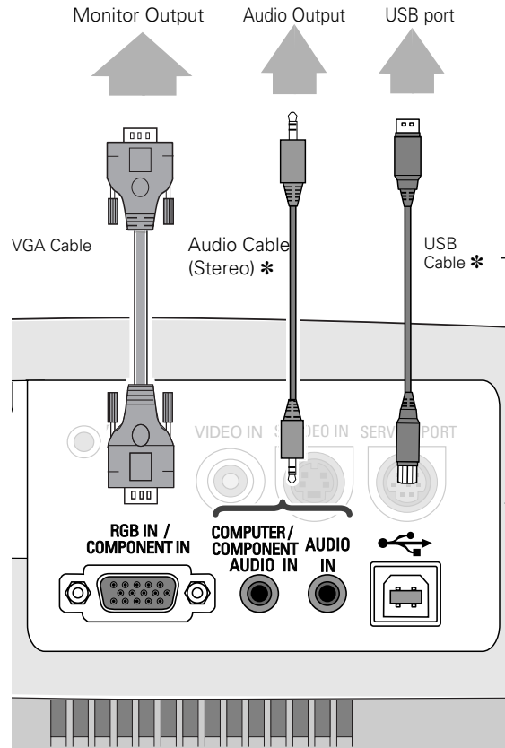
Terminals of the Projector
