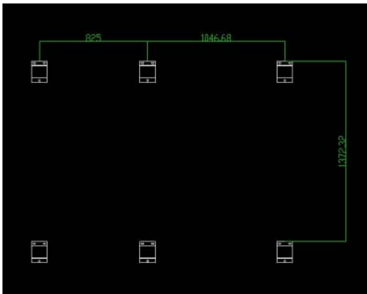
Back bracket fixing angle code (each secured with 3 x M8 expansion screws)
