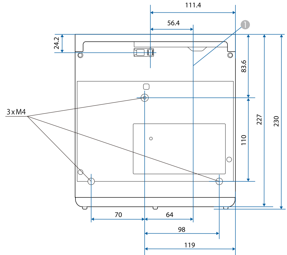
2 Distance from center of lens to suspension bracket fixing point
